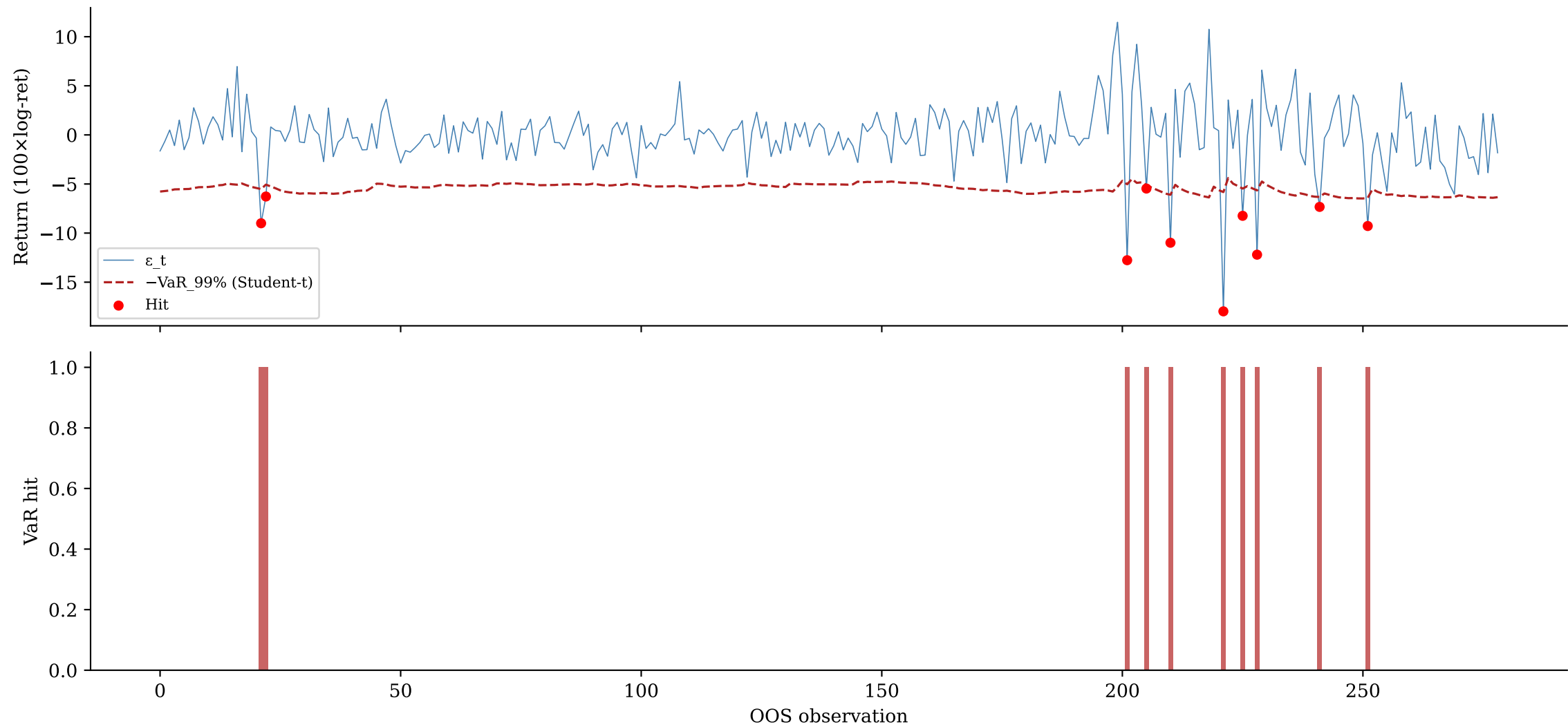
LSTM-SSE-t-Student — OIL VaR 99% Hit Sequence
